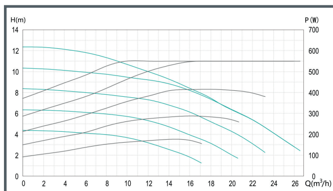
WITA go.max F 50-12F-280
